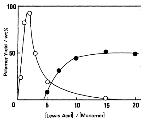
Fig. 5. Effect of the concentration of Lewis acid on the polymerization of diphenyl disulfide. AlCl 3 (●), SbCl 5 (○).
